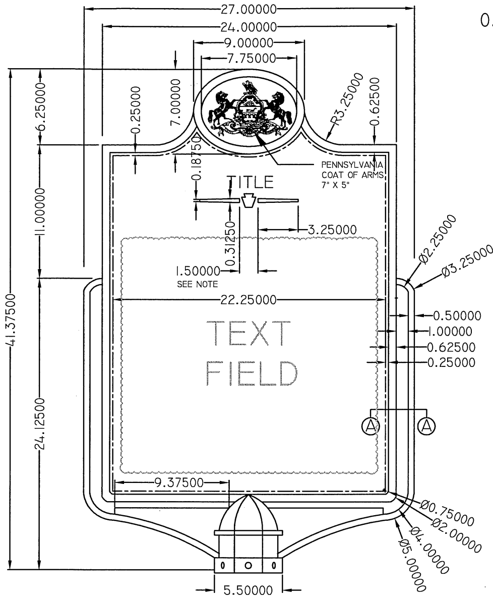
FRONT VIEW SCALE: 1.5" = 1.0'
